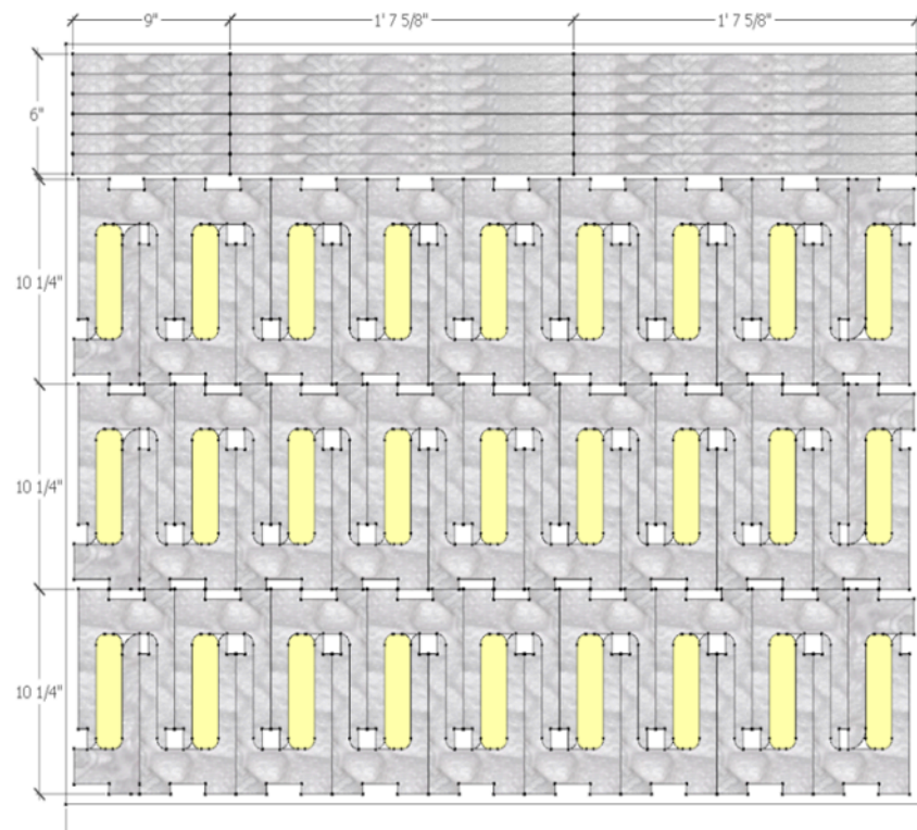
Figure 4. Optimized Cutting Pattern
